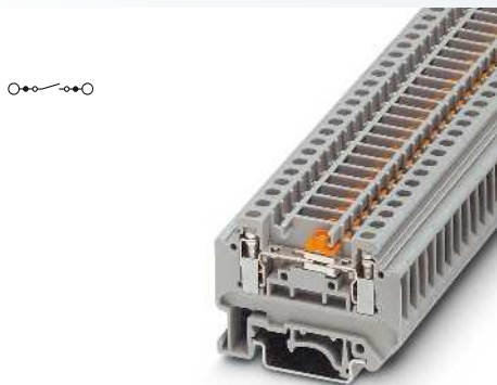
4 (4) mm², 26 A, test disconnect terminal block
