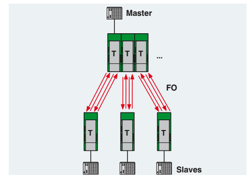
Redundant structure
