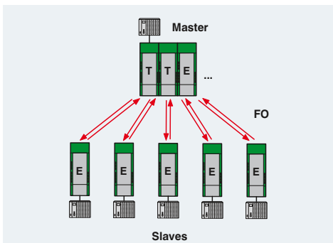
Star structure
