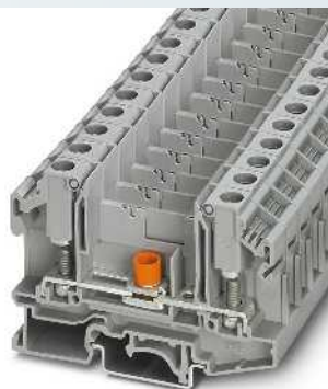
6 (6) mm 2 , 41 A, test disconnect terminal block, with test socket screws, for accommodating switching jumpers
