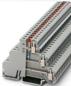
2.5 (4) mm 2 , 30 A, three-level terminal block with LED display
