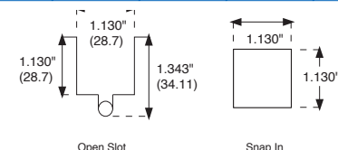
PANEL CUTOUT
