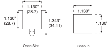
PANEL CUTOUT
